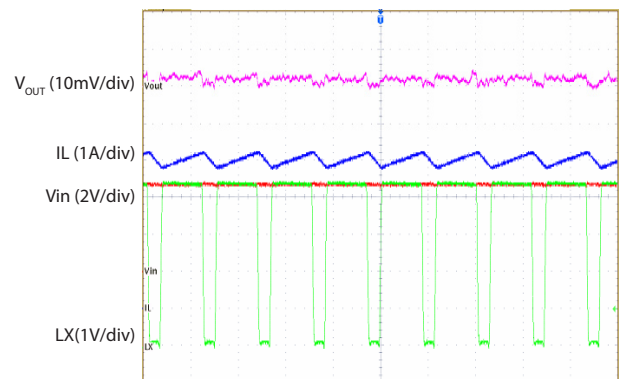
Vout Ripple ( V_{in}=5\text{V} , V_{OUT} = 3.3\text{V} ) @ Full Load
