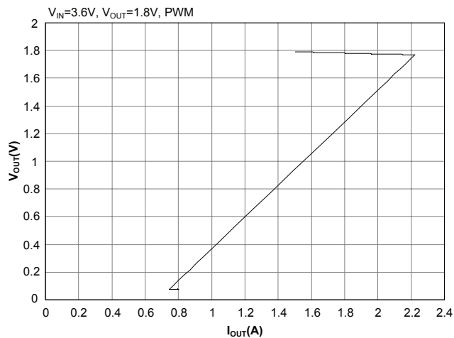
Current Limit
