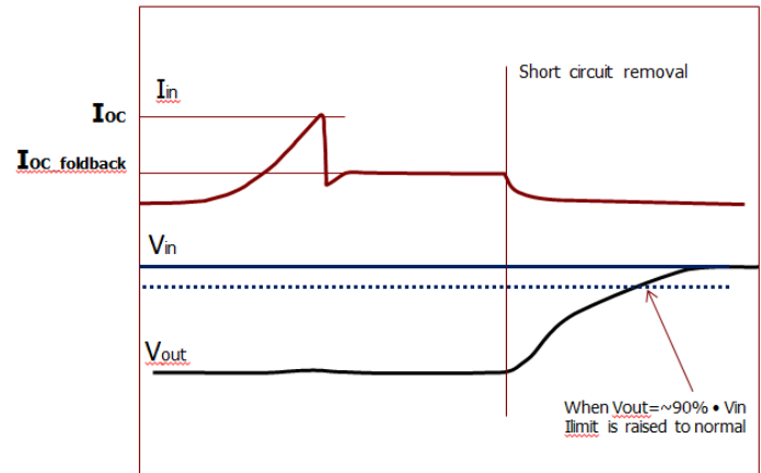
Figure 1 — Startng into Short Circuit and Recovery from Short Circuit Removal Behavior
