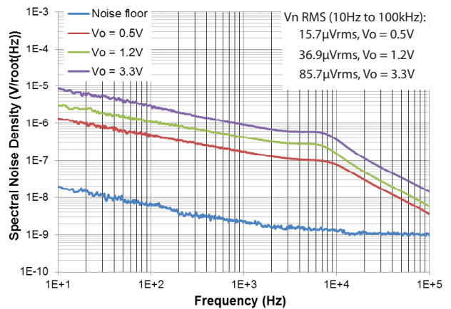
Output Spectral Noise Density \text{CBYP} = 470\text{nF} , \text{RL} = 50\Omega
