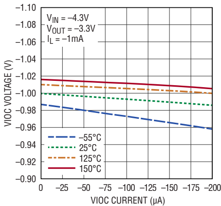
VIOC Voltage
