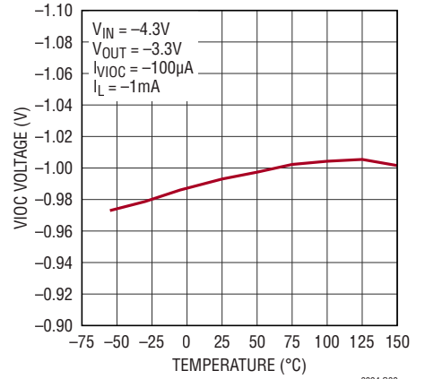
VIOC Voltage
