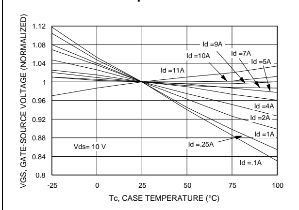
Figure 7. Gate-source voltage vs case temperature
