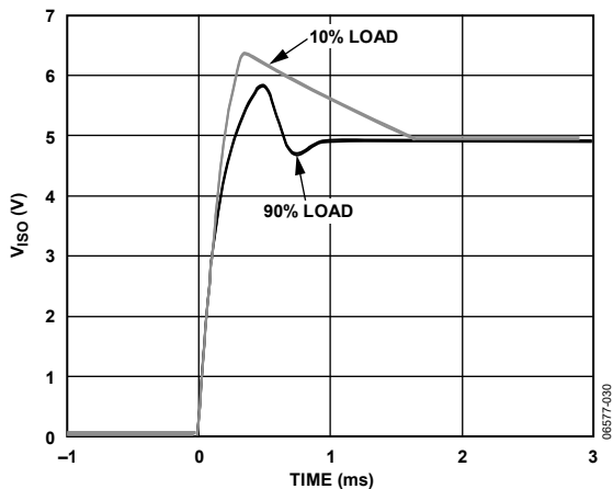
Figure 19. Typical Output Voltage Start-Up Transient at 10% and 90% Load, V_{ISO} = 5\text{ V}
