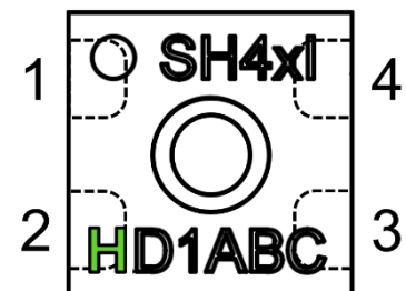
Figure 10: Pin assignment (transparent top view). Dashed lines are only visible if sensor is viewed from below. The die pad is not directly connected to any pin. The laser marking consists of two lines, indicated in Figure 8 and Figure 10 . In the first line a filled circle serves as pin-1 indicator and is followed by “SH4”. The fourth character will indicate the accuracy class of this product (here “x” serves as place holder). Lastly, “I” indicates the industrial grade. In the second line, the first three characters specify the product characteristics according to positions 7, 8 and 9 of Table 11 . The second three characters serve as internal batch tracking code.
