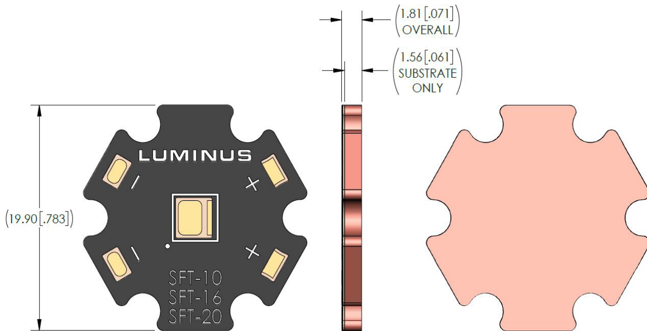
FRONT SIDE
