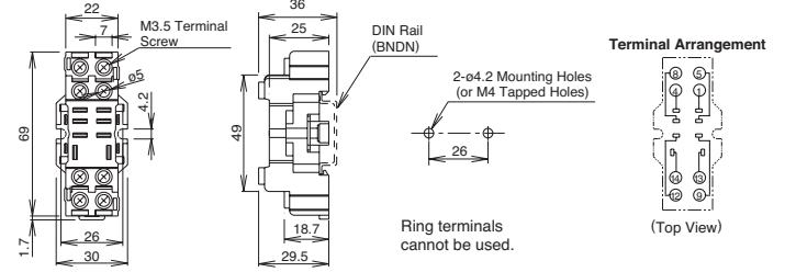
SH2B-05C
