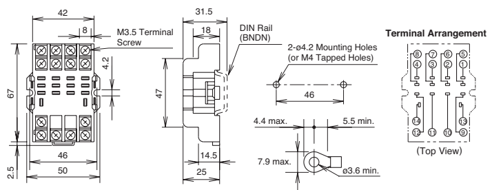
SH4B-05
