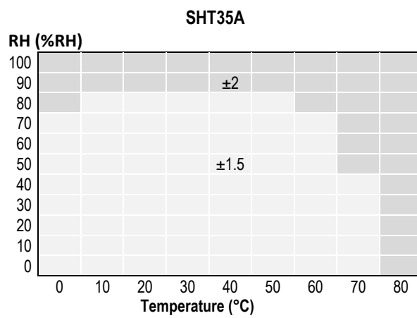
Figure 7 Typical tolerance of RH over T for SHT35A.
