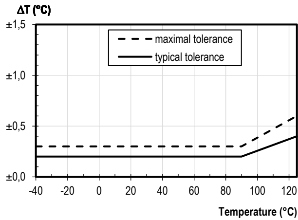
Figure 10 Temperature accuracy for SHT35A.
