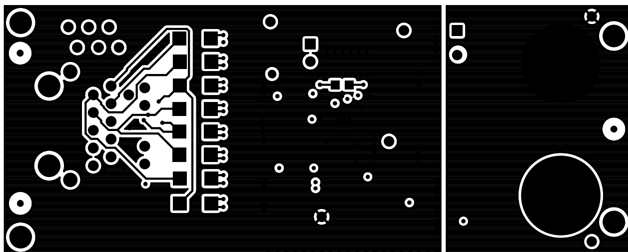
Figure 8.5. Bottom Layer
