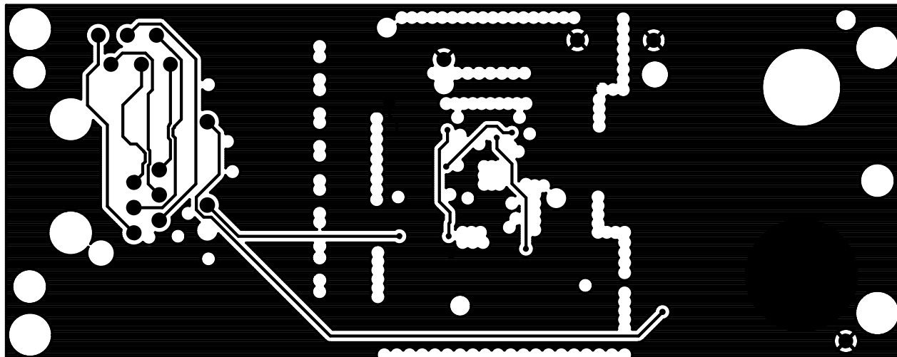
Figure 8.4. Internal 2 (Layer 3)
