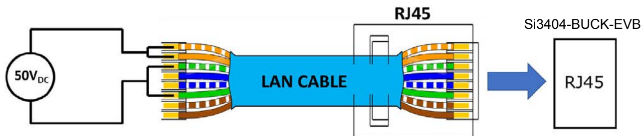
Figure 2.2. Midspan Connection using Laboratory Power Supply
