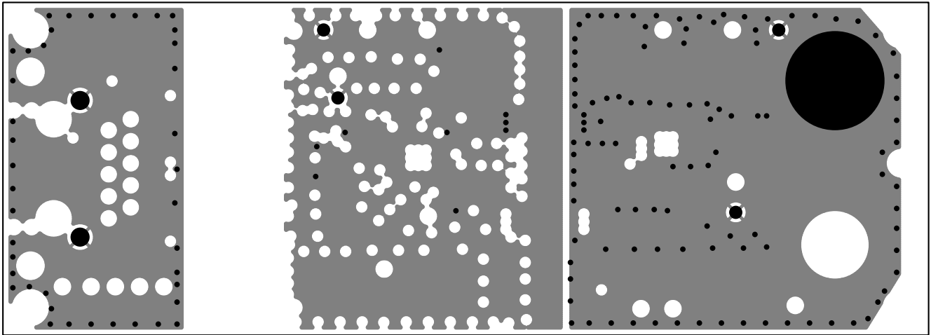
Figure 65. Internal 1 (Layer 2)
