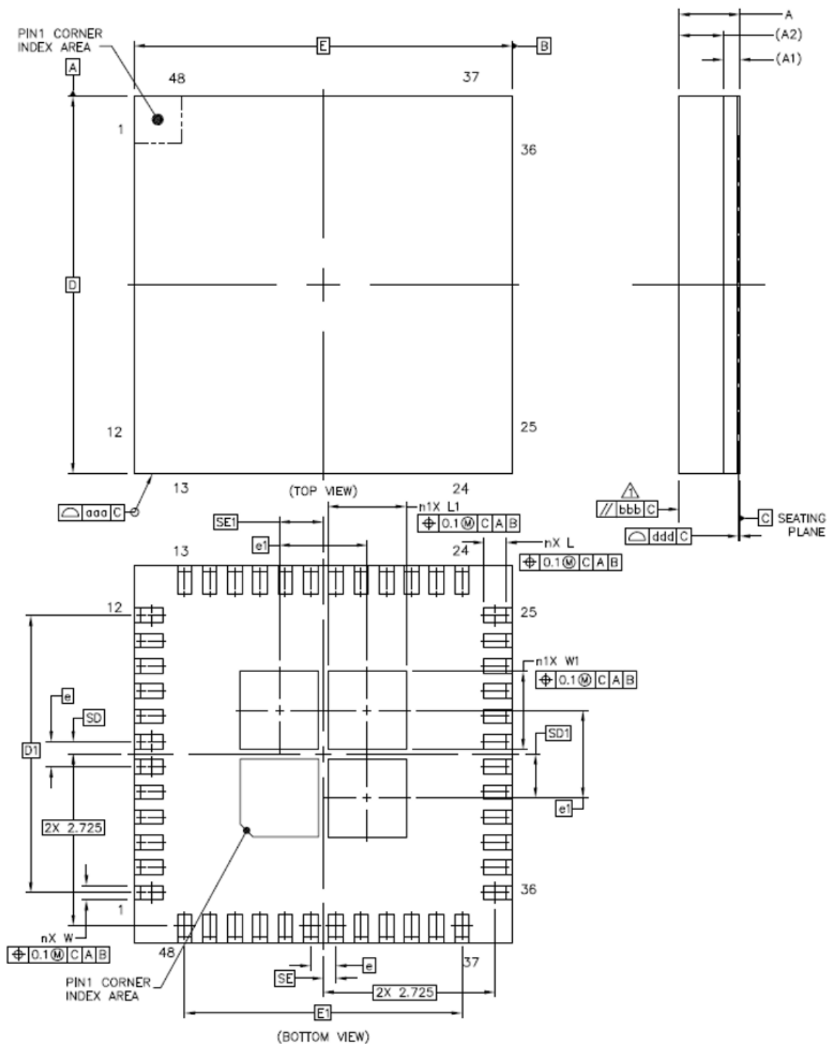
Figure 7.4. 48-Pin LGA
