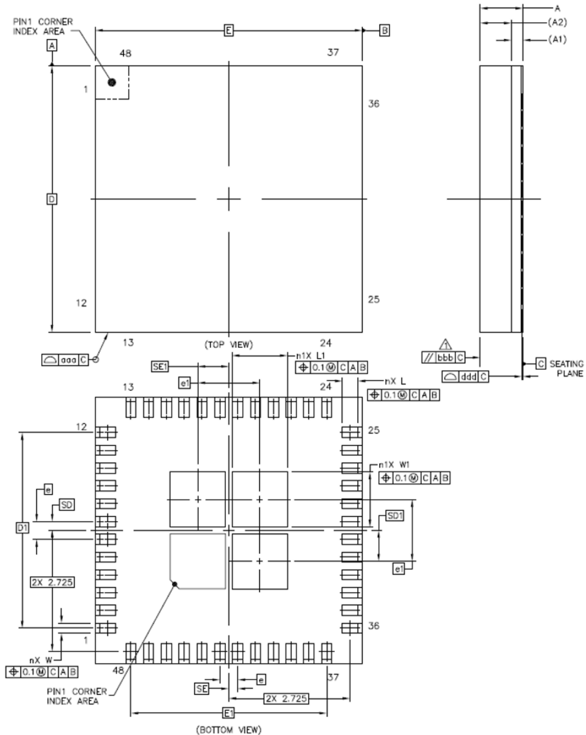
Figure 7.4. 48-Pin LGA
