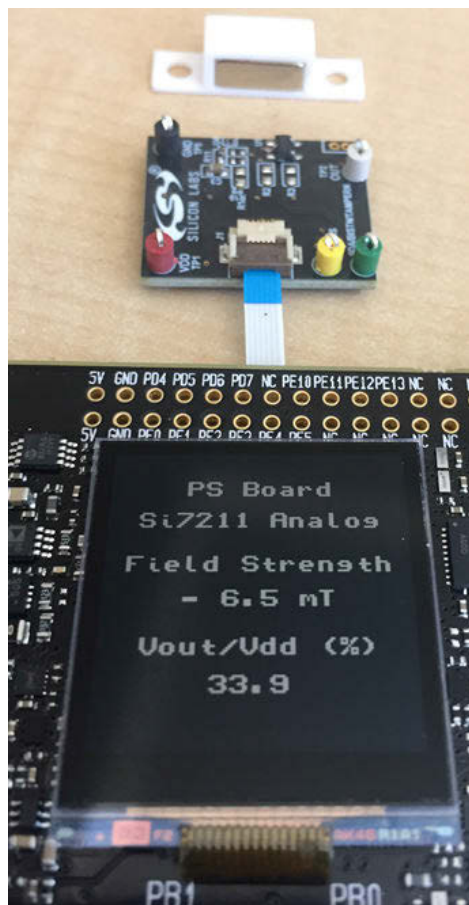
Figure 1.10. Analog Out Screen
