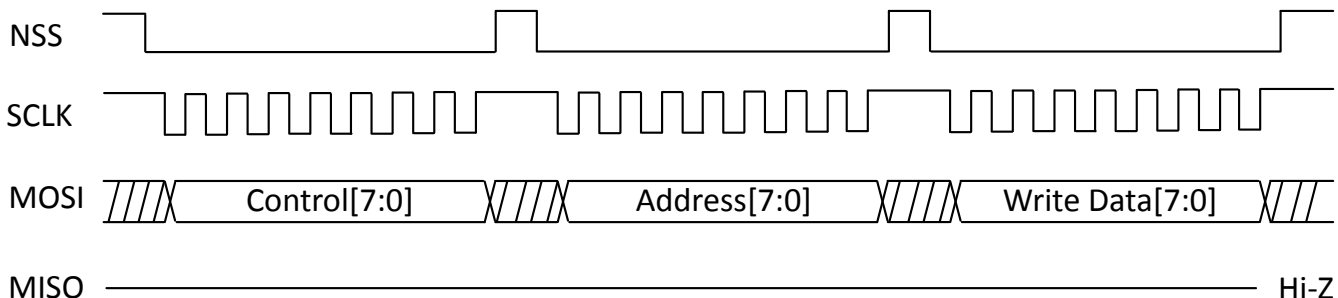
Figure 3.6. SPI Write Operation
