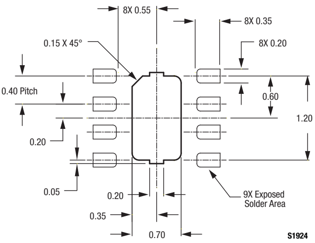
Figure 10. SKY13317-373LF PCB Layout Footprint (Top View)
