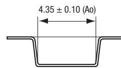
Figure 12. SKY13372-467LF Tape and Reel Dimensions
