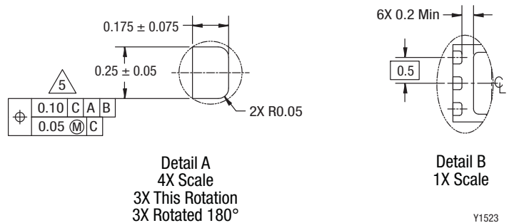
Figure 13. SKY13411-374LF 6-Pin QFN Package Dimensions
