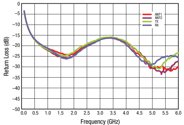
Figure 6. Return Loss vs Frequency,
