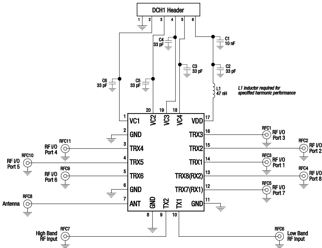
Figure 15. SKY13441 Evaluation Board Schematic
