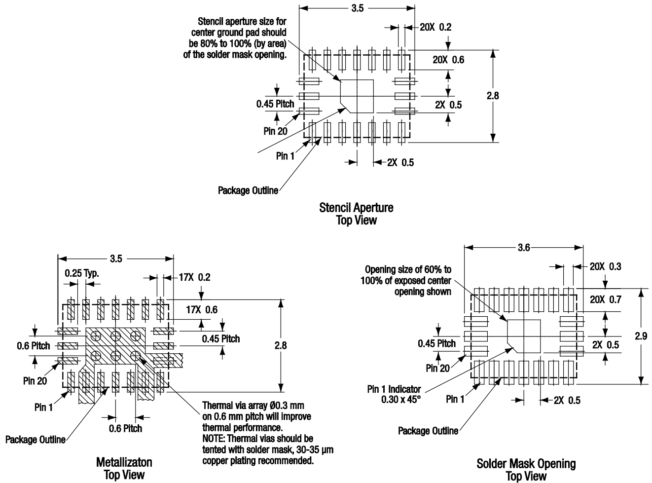
Figure 18. SKY13441 PCB Layout Footprint (Top View)
