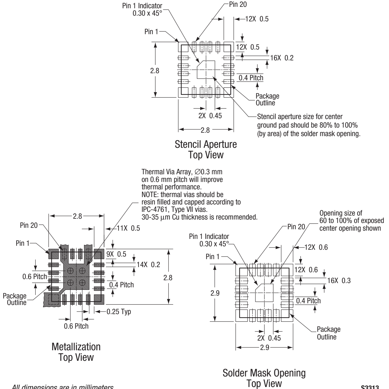
Figure 10. SKY13488-21 PCB Layout Footprint (Top View)
