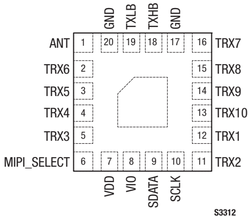
Figure 2. SKY13488-21 Pinout – 20-Pin MCM (Top View)
