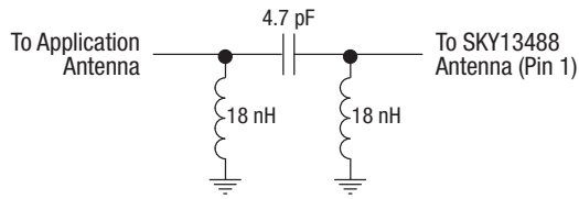
ESD Circuit 1
