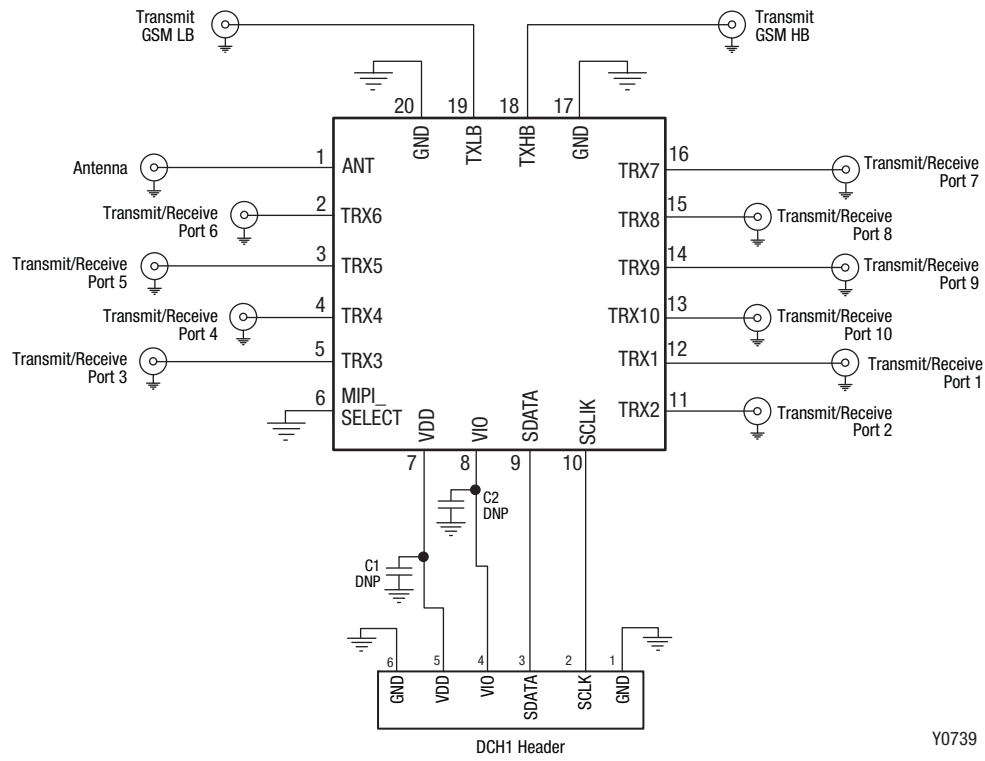
Figure 7. SKY13488-21 Evaluation Board Schematic
