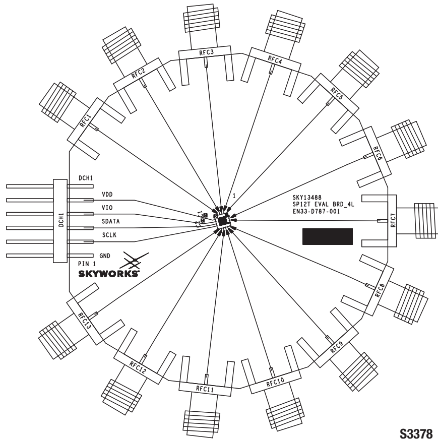
Figure 9. SKY13488-21 Evaluation Board Assembly Diagram
