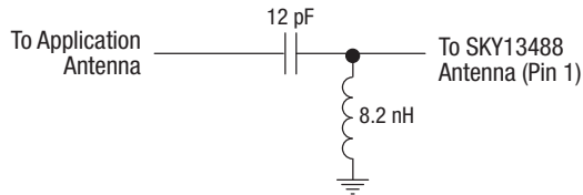
ESD Circuit 2
