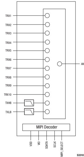
Figure 1. SKY13488-21 Block Diagram
