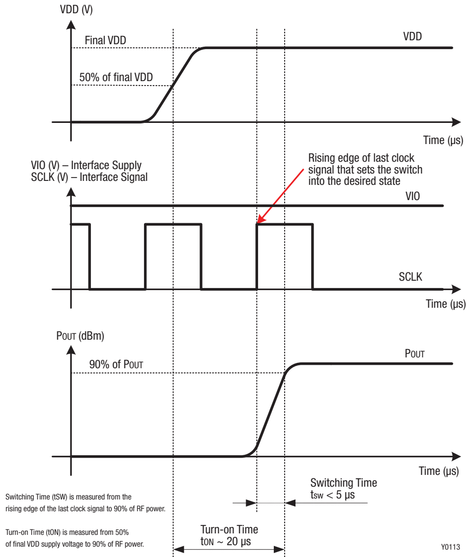
Figure 3. SKY13488-21 Timing Diagram
