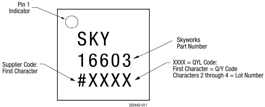
Figure 10. SKY16603-632LF Typical Part Markings
