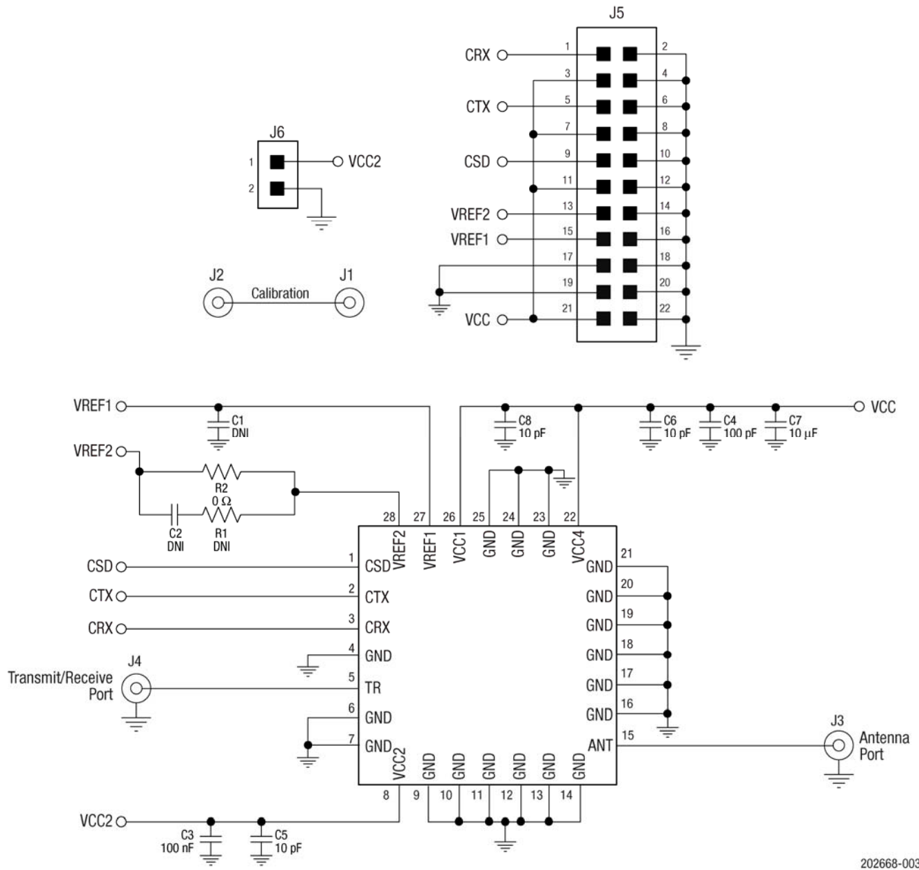
Figure 3. SKY65383-11 Typical Application Schematic
