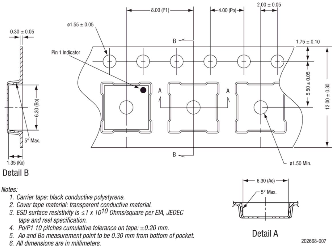
Figure 7. SKY65383-11 Tape and Reel Dimensions
