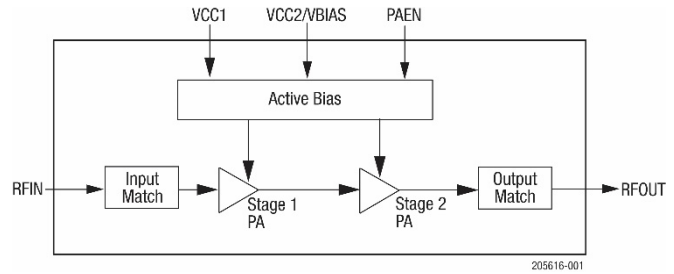
Figure 1. SKY66042-11 Block Diagram
