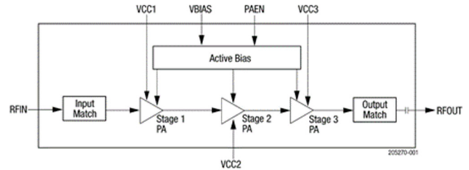
Figure 1. SKY66320-11 Block Diagram
