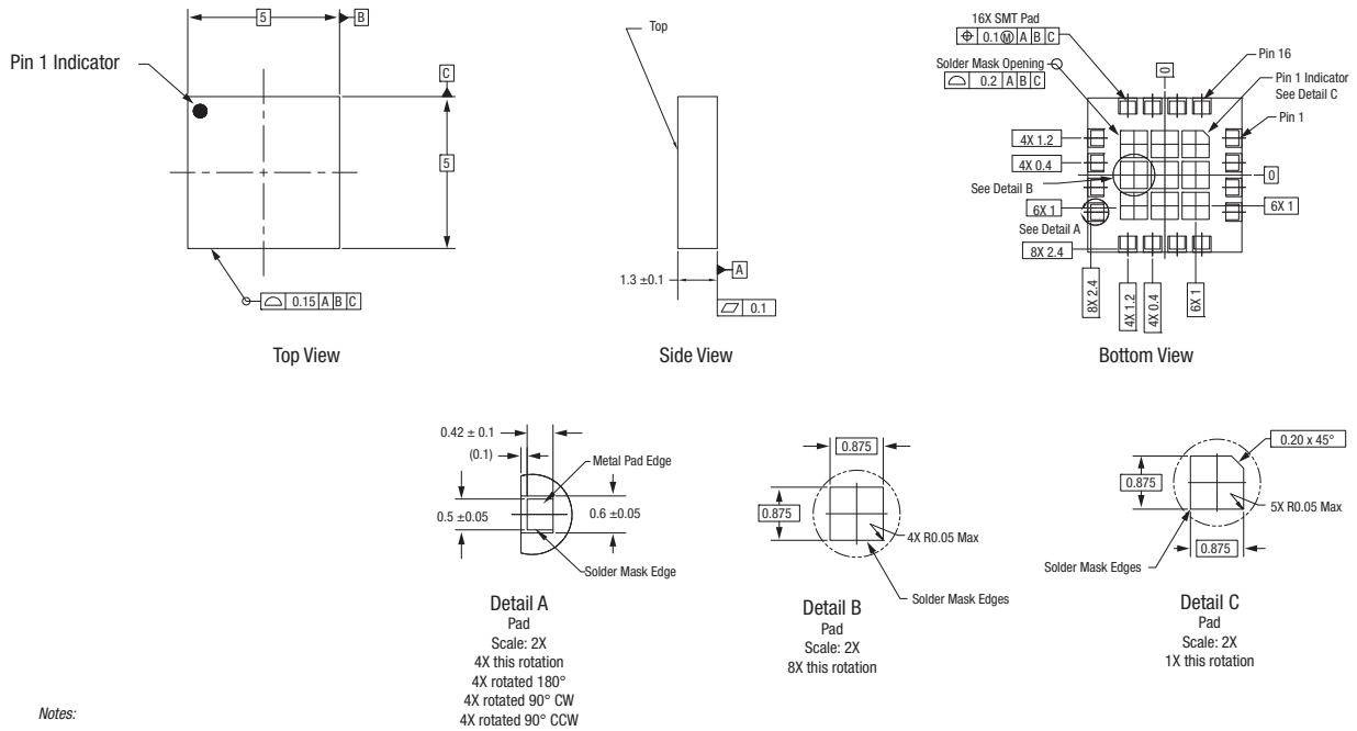
Figure 23. SKY66394-11 Package Dimensions
