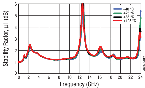
Figure 12. Stability Factor ( \mu_1 ) vs Frequency Over Temperature
