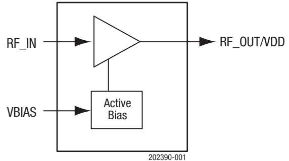
Figure 1. SKY67151-396LF Block Diagram
