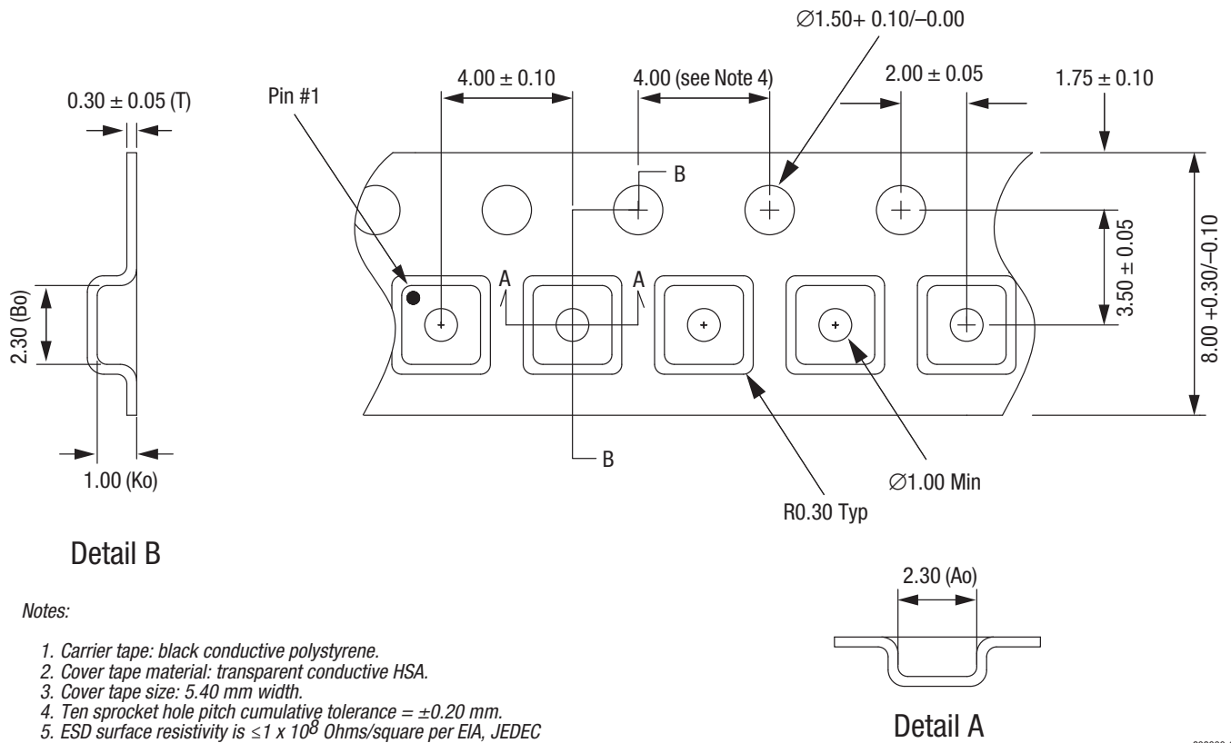
Figure 28. SKY67151-396LF Tape and Reel Dimensions
