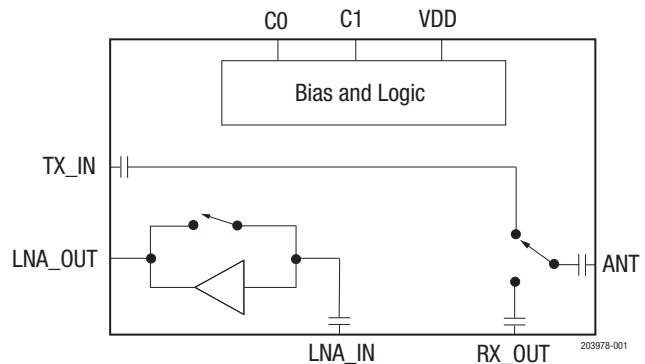
Figure 1. SKY85216-11 Block Diagram
