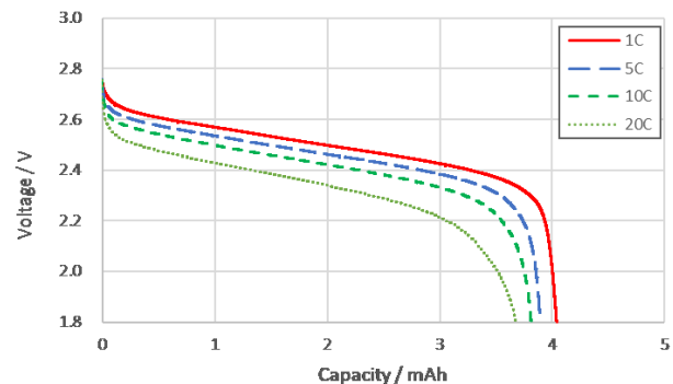
Discharge characteristics
