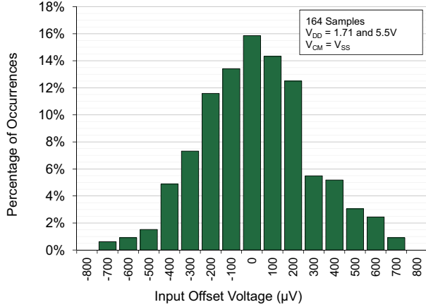
Fig 1. Input Offset Voltage Distribution V_{CM} = V_{SS} ; V_{DD} = 1.71\text{ V} and 5.5\text{ V} ; T_A = 25^\circ\text{C} .
