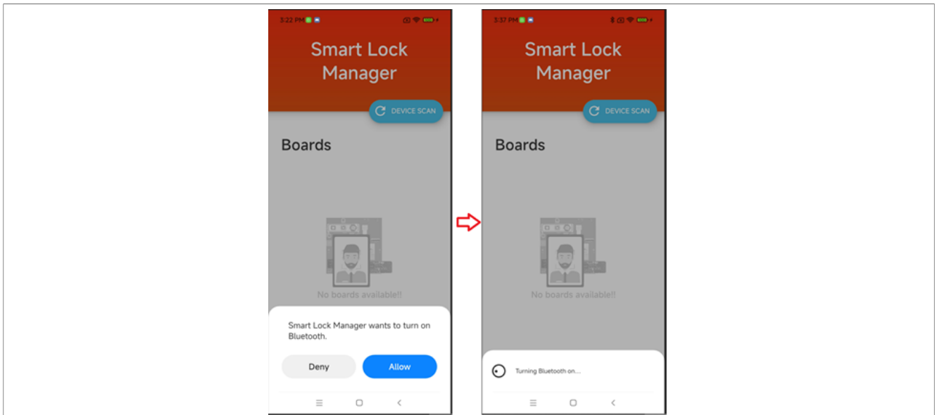
Figure 18. Enabling Bluetooth
