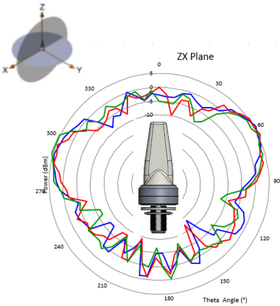
Elevation Plane
