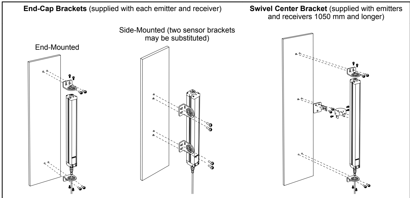
Figure 10. Sensor brackets
