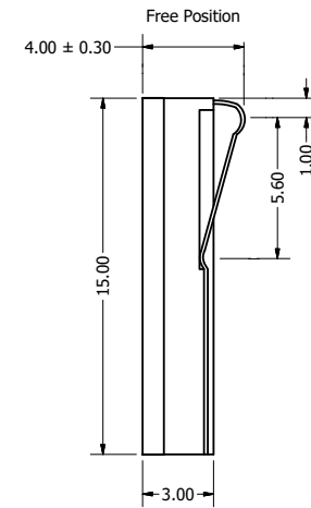
Side View (1)
