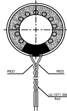
BOTTOM VIEW
