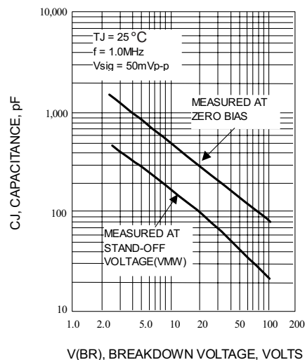
Fig. 4-TYPICAL JUNCTION CAPACITANCE
