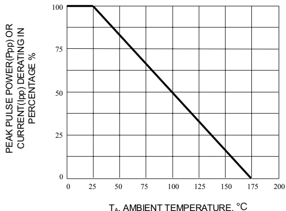
Fig. 2-PULSE RATING CURVE
