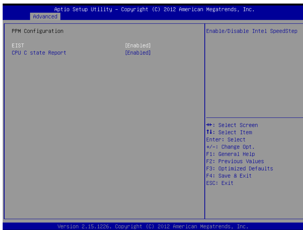
Figure 3.13 PPM Configuration
