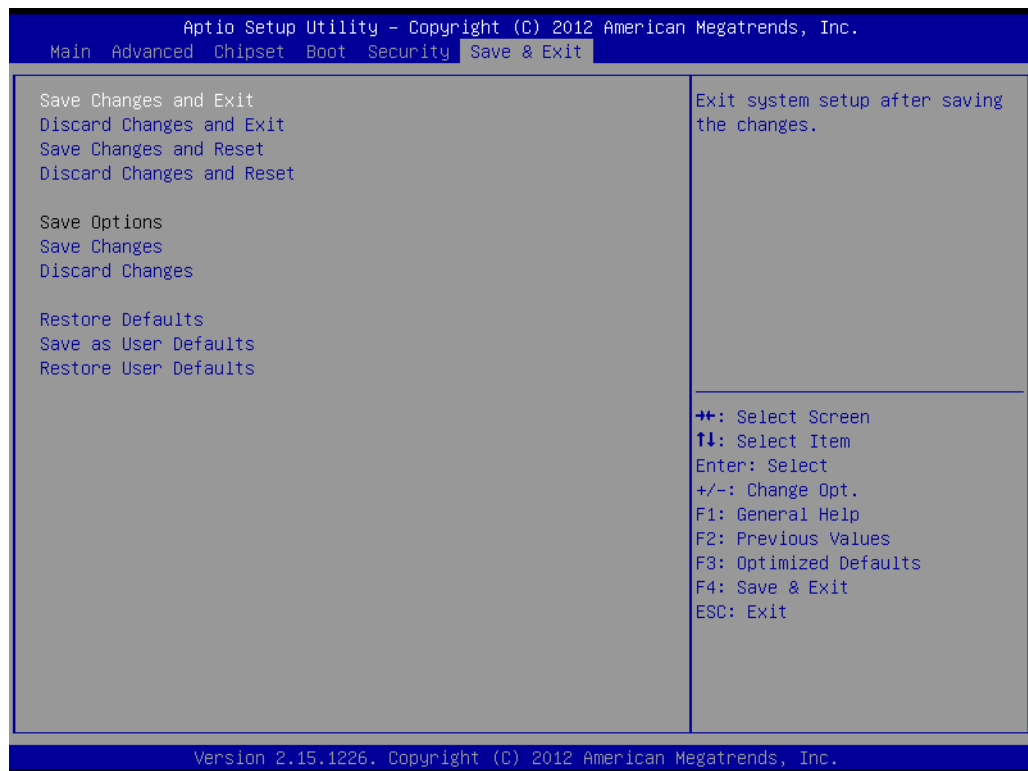
Figure 3.24 Save & Exit
