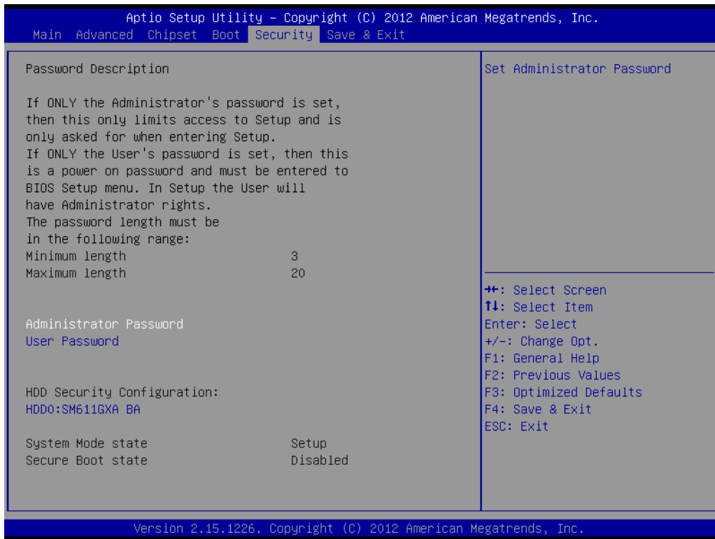
Figure 3.23 Password Configuration
