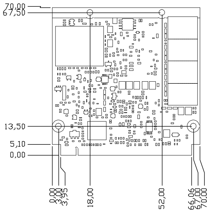
Figure 2.4 Board Mechanical Drawing - Back
