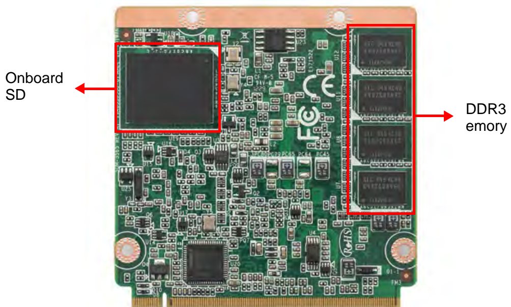
Figure 2.2 Board Chip Placement - Back
