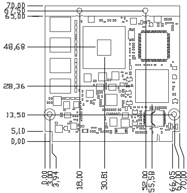
Figure 2.3 Board Mechanical Drawing - Front
