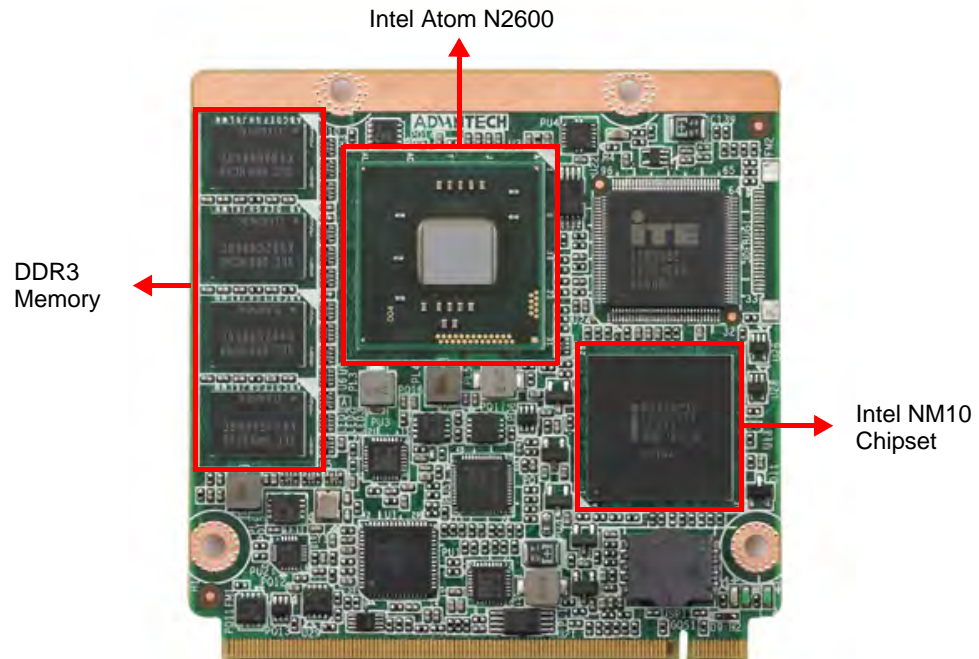
Figure 2.1 Board Chip Placement - Front
