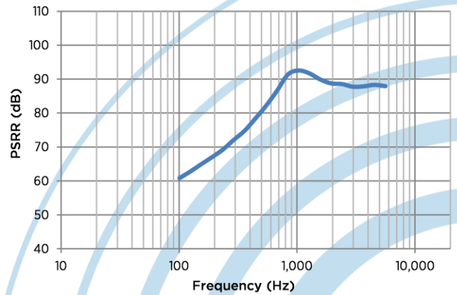
Figure 11: Typical PSRR (NM)
