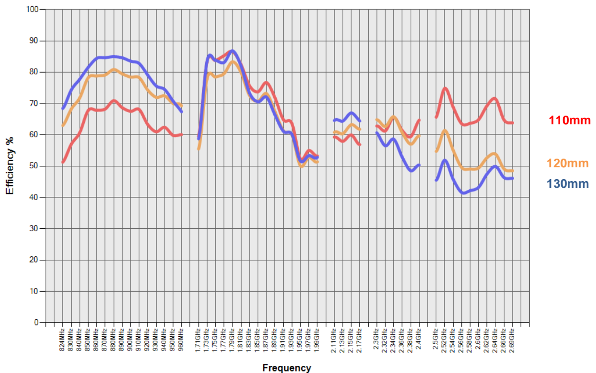
Passive Efficiency vs. PCB length All results measured in Antenova's anechoic chamber
