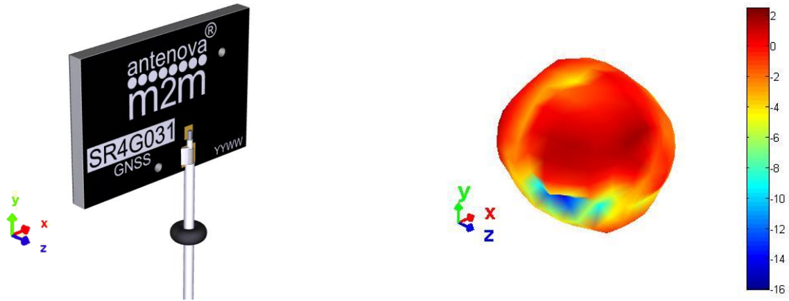
3D pattern at 1575.4 MHz Drag to rotate pattern and PCB by using Adobe Reader (Click to Activate)
