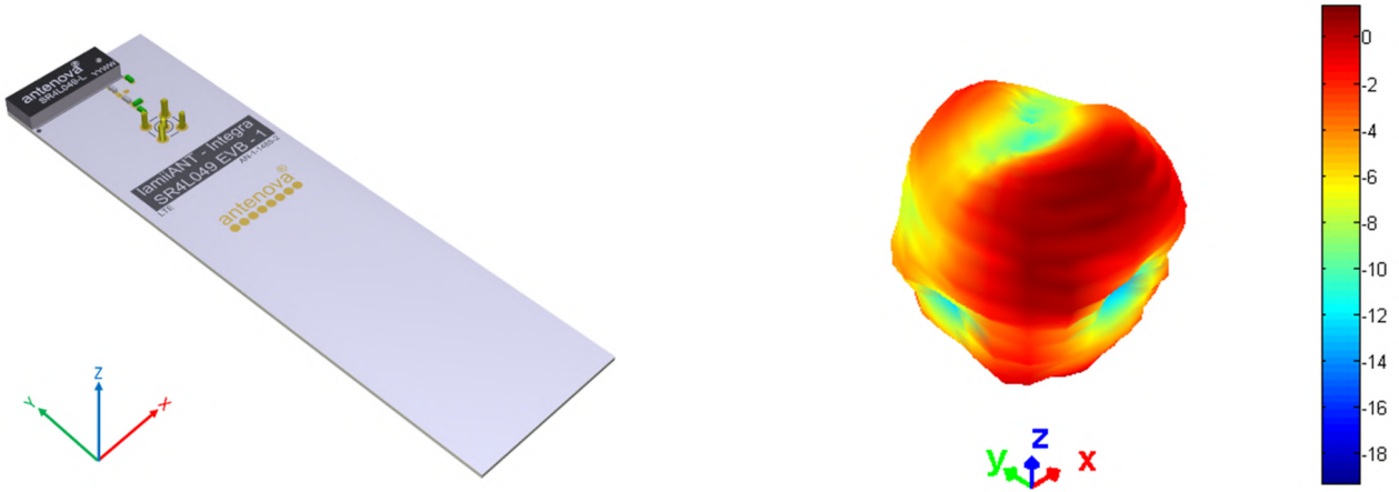
3D pattern at 1990MHz
