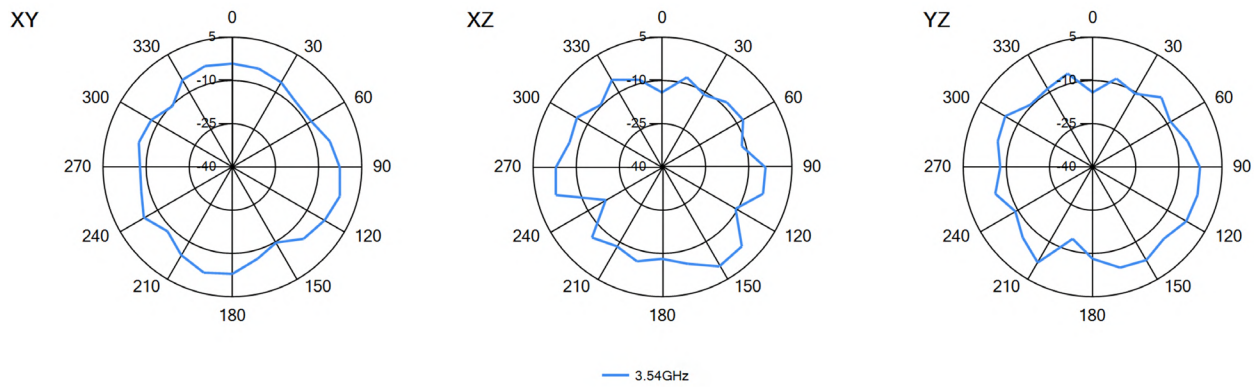
3D pattern at 3540MHz
