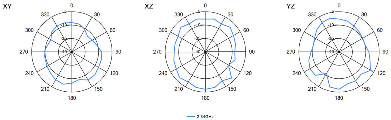
3D pattern at 2340MHz
