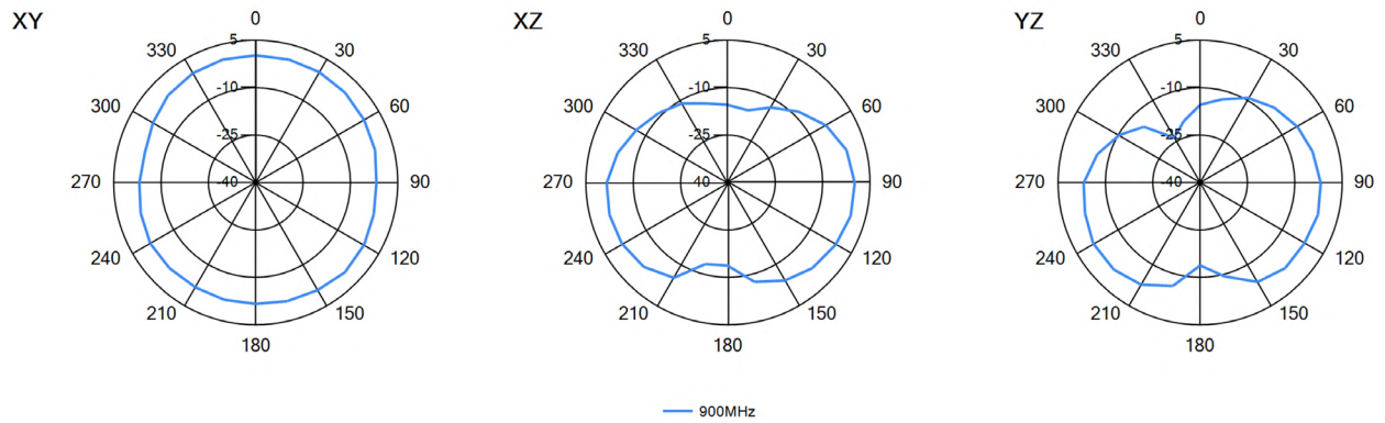
3D pattern at 900MHz
