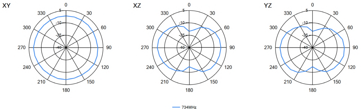
3D pattern at 734MHz
