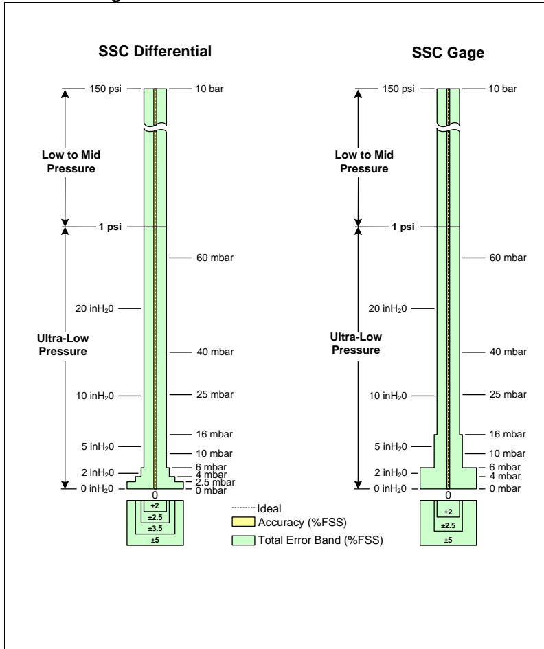
Figure 4. SSC Series Total Error Band Values for Full Scale Span Pressure Ranges
