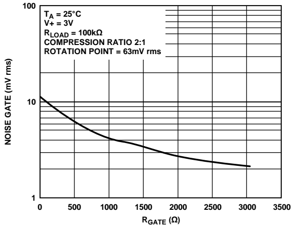
Figure 3. Noise Gate vs. R_{\text{GATE}}
