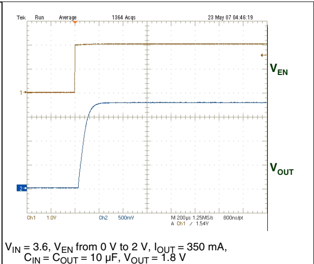
Figure 25. Enable transient
