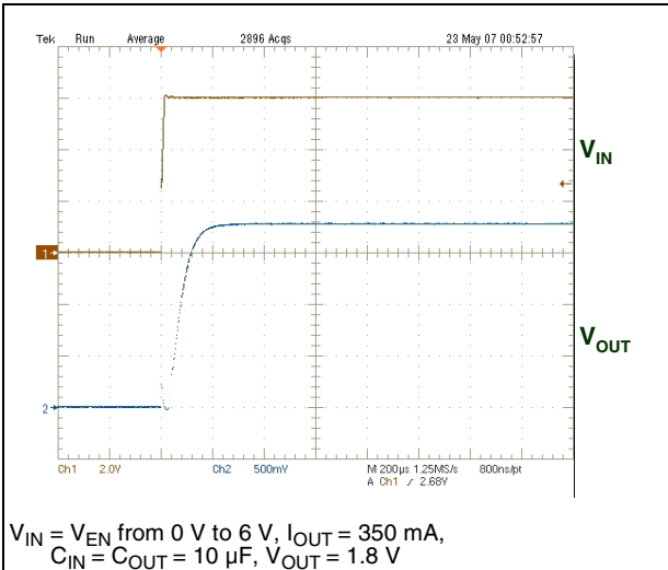
Figure 24. Start-up transient
